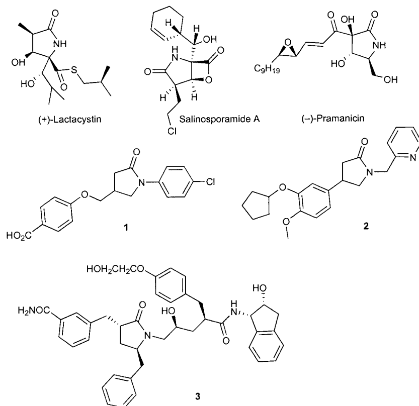
Figure 1. Examples of natural and synthetic \gamma -lactam derivatives.
