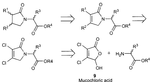
Scheme 1. Retrosynthetic analysis.
