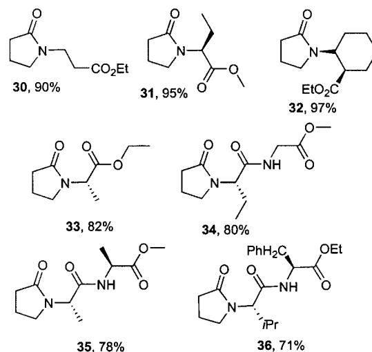
Scheme 4. Products from dehalogenation of the \alpha,\beta -unsaturated \gamma -lactams.
