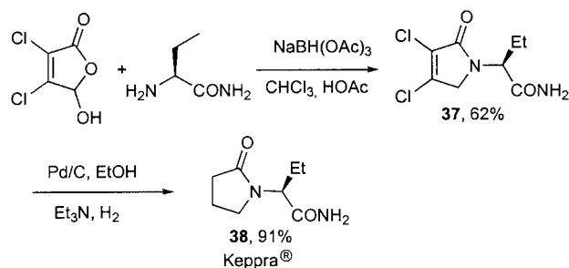
Scheme 5. Synthesis of Keppra® from mucochloric acid.
