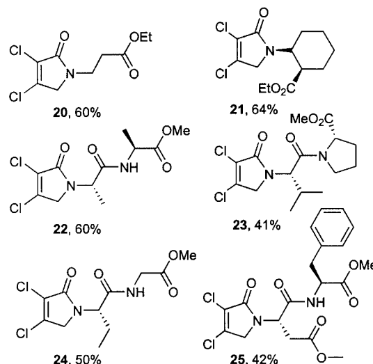
Scheme 2. Reductive amination with \beta -amino acids and peptides.
