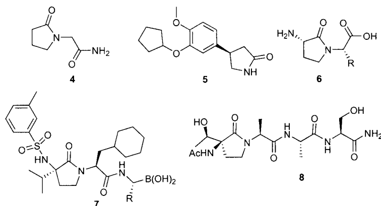
Figure 2. Examples of \gamma -lactam-containing short peptides.
