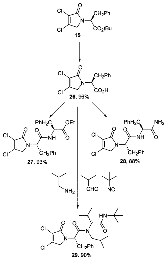
Scheme 3. Application of the reductive amination product in peptide coupling and peptoid synthesis.
